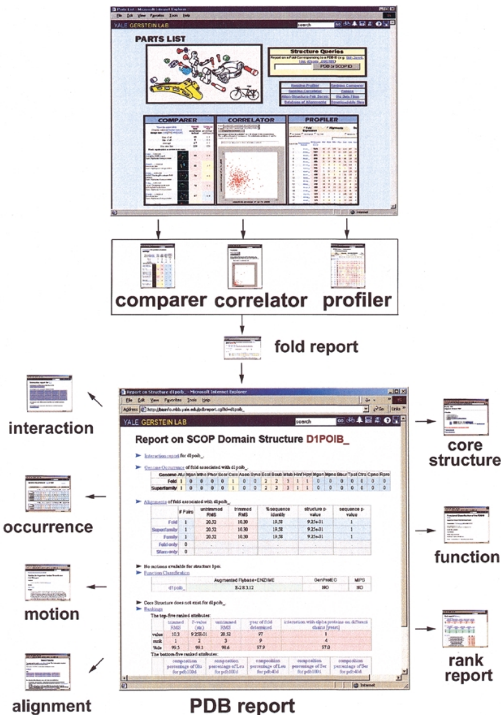
Figure 1. The overall structure of PartsList. Three tools (Profiler, Comparer and Correlator) provide an easy way to access and manipulate the display of the dataset. With these tools, users can isolate interesting folds and obtain fold reports about them. Further clicks take one to PDB report, which gives detailed information about an individual structural domain, including its genome occurrence, alignment information, molecular motions, functional annotation, interactions and core structure.
